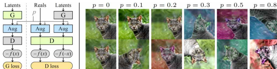
Figure 7.8: StyleGAN2 ADA Training
