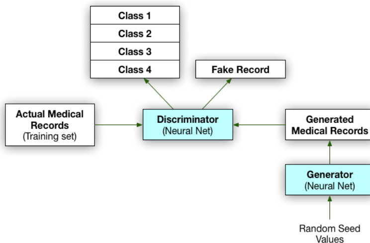
Figure 7.13: GAN for Semisupervised Training
