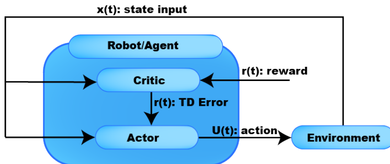
Figure 12.4: Actor Critic Model
