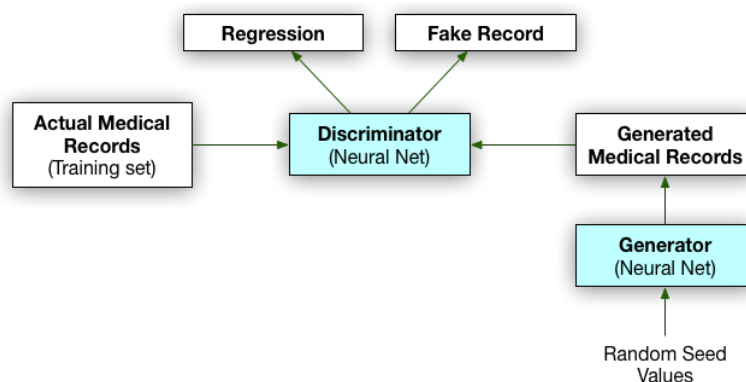
Figure 7.15: Semisupervised Structure.
