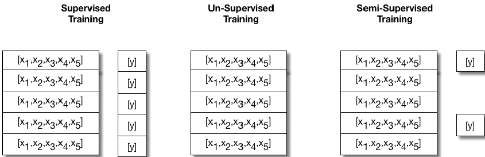
Figure 7.12: Supervised, UnSupervised and Semi-Supervised
