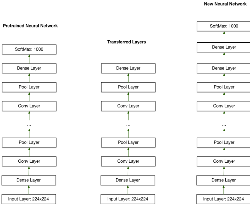
Figure 9.1: Transfer Learning
