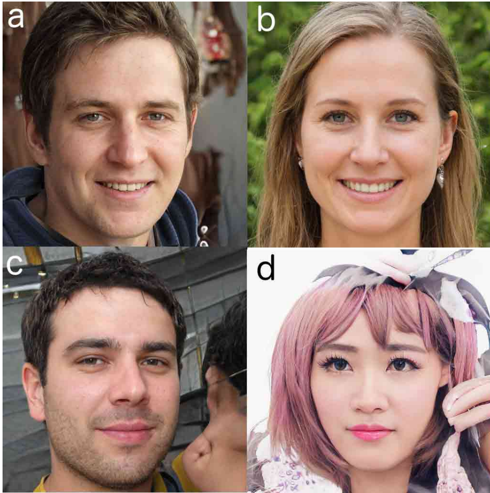
Figure 7.9: StyleGAN2 Face
