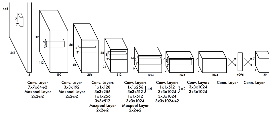
Figure 6.12: YOLO Structure
