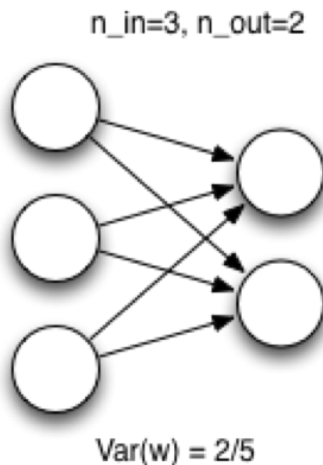
Figure 3.20: Xavier Weight Initialization
